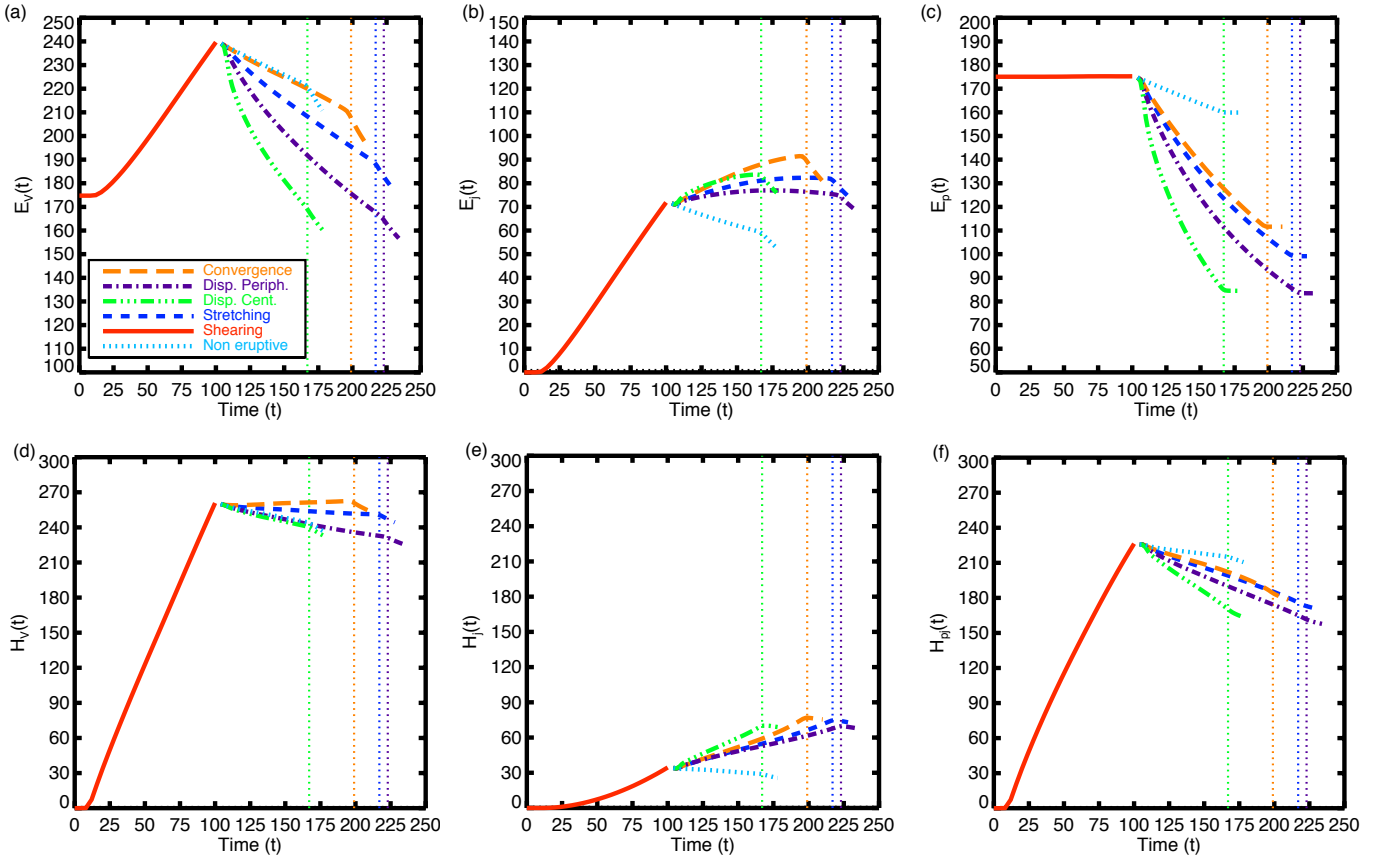
FIG. 4.— Time evolution of the different energy (top) and helicity (bottom) terms for the shearing and flux rope formation phases.
