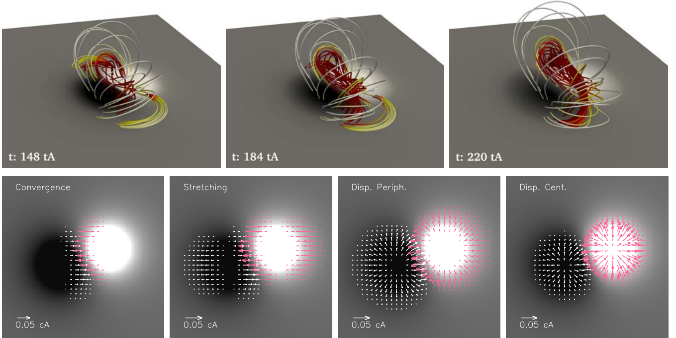
FIG. 2.— Evolution of the magnetic field for the Dispersion Peripheral run during the flux rope formation phase (top panels) and the applied boundary motions (bottom panels) for the four different simulations runs. Colour scheme is the same as Figure 1.
